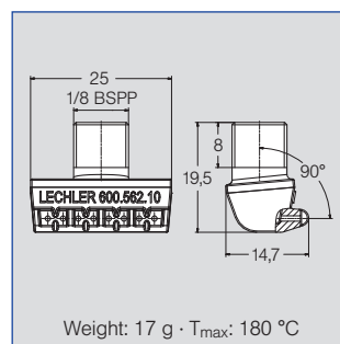
600. 562. 1Y. 10 (Stainless steel 316L)
