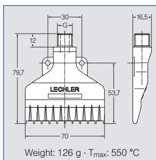
600. 493. 1Y (Stainless steel 316L)
